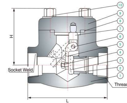
Bolted Bonnet
